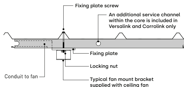
PANEL END VIEW OF SPACEMAKER
